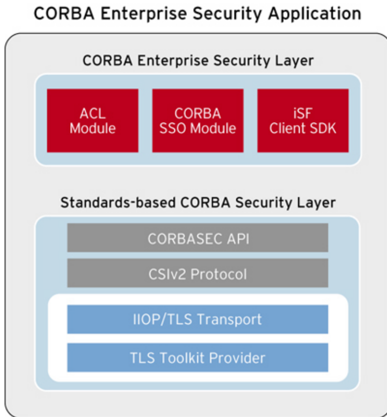
Figure 4: Architecture of Orbix CORBA server application that has been security enabled.
