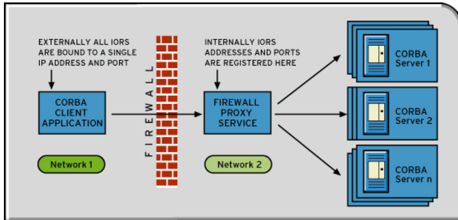
Figure 8: Firewall Proxy Service
