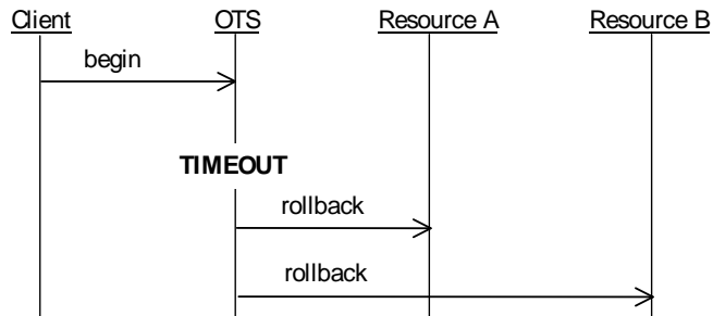
Figure 7: Rollback after a timeout
