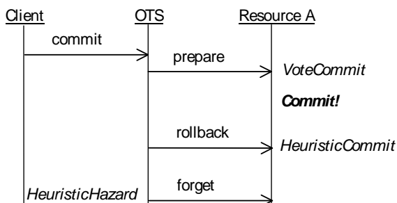
Figure 13: Raising the HeuristicCommit exception
