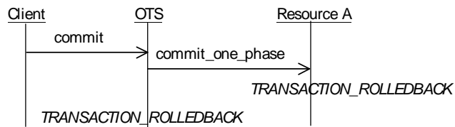
Figure 12: The IPC protocol resulting in a rollback.
