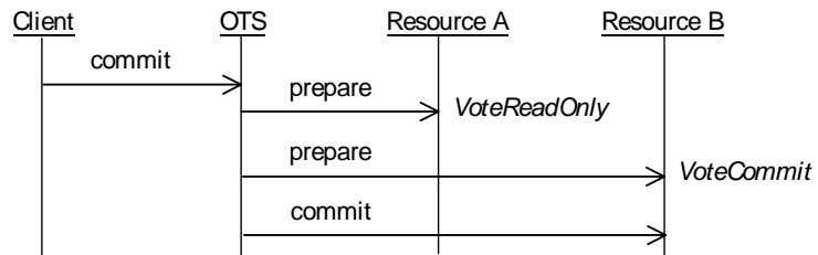
Figure 10: A resource returning VoteReadOnly .
