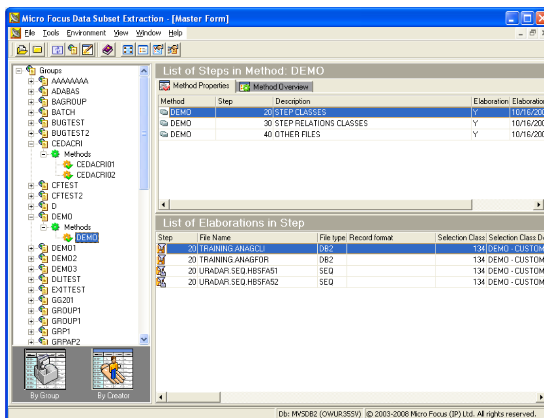
Figure 5-1: Data Subset Extraction – [Master Form] Window
