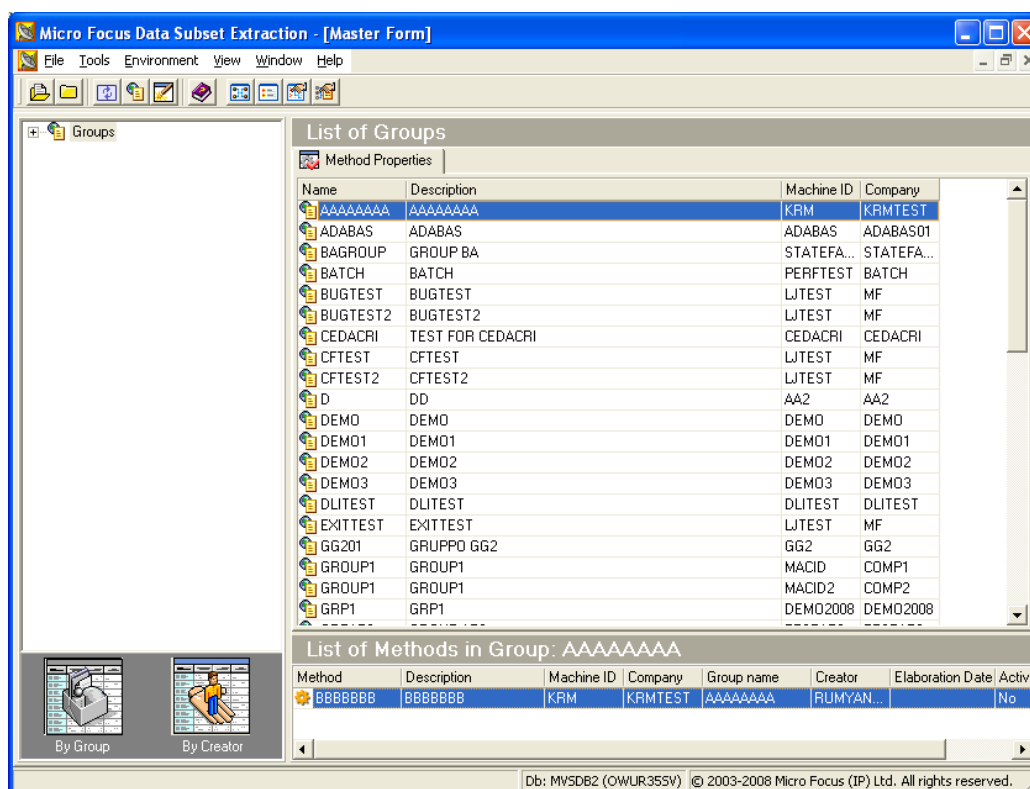
Figure 4-1: Data Subset Extraction - [Master Form] Window
